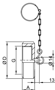
带链条盲螺母 Blind Cap with Chain
